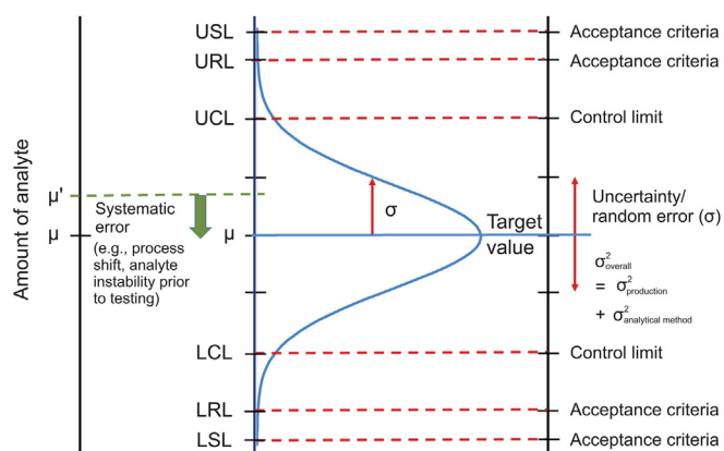
Fig. 4. Control limits of the manufacturing process and acceptance criteria (release limits and specification limits) of the specification. \mu and \mu' : population mean; \sigma , population standard deviation; \sigma^2 : population variance; LCL: lower control limit; LRL: lower release limit; LSL: lower specification limit; UCL: upper control limit; URL: upper release limit; USL: upper specification limit.
